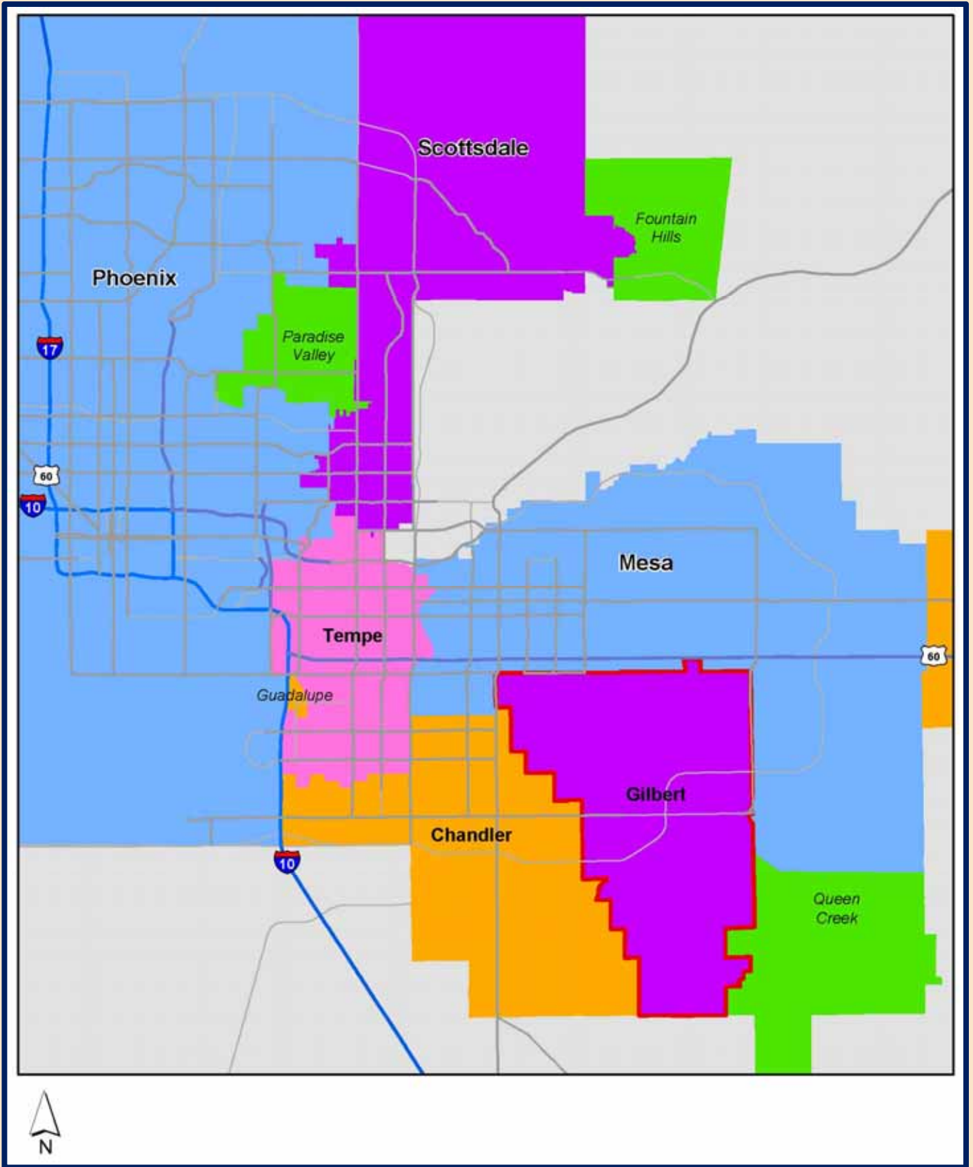
FIGURE 1-1: VICINITY MAP
