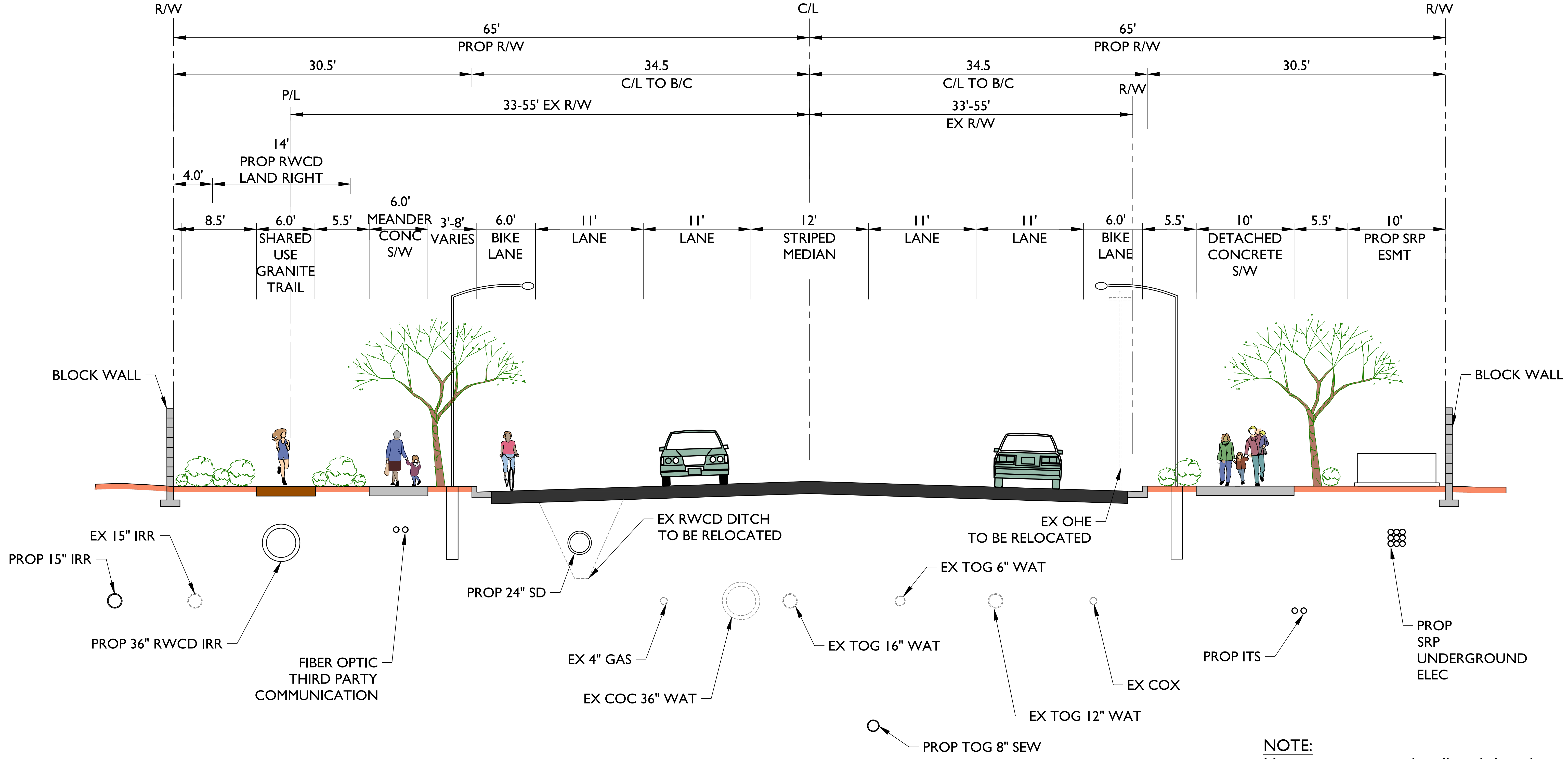
OCOTILLO ROAD VAL VISTA DR TO GREENFIELD RD TYPICAL SECTION (LOOKING EAST)
