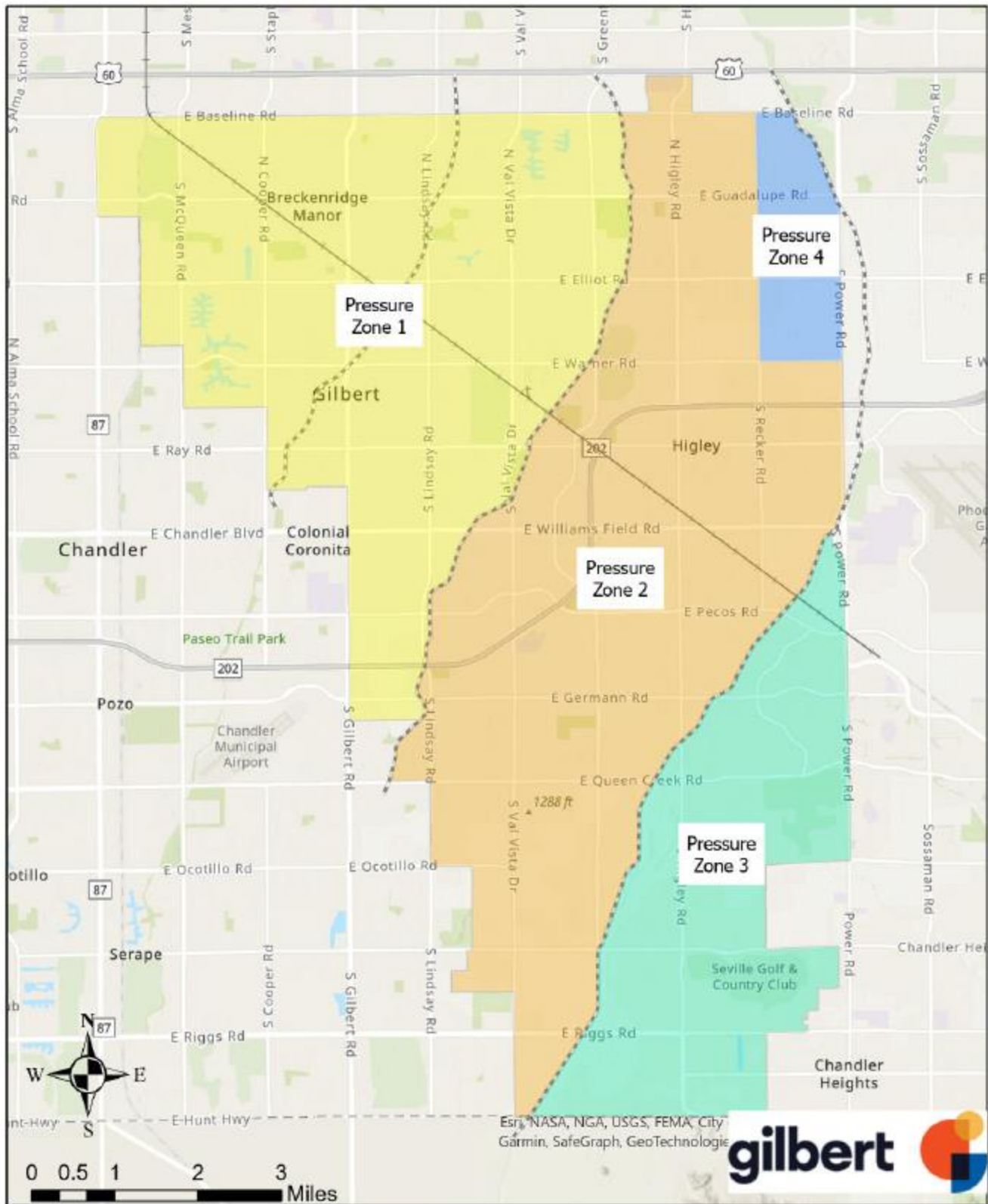
FIGURE 7-1 WATER SYSTEM PRESSURE ZONES
