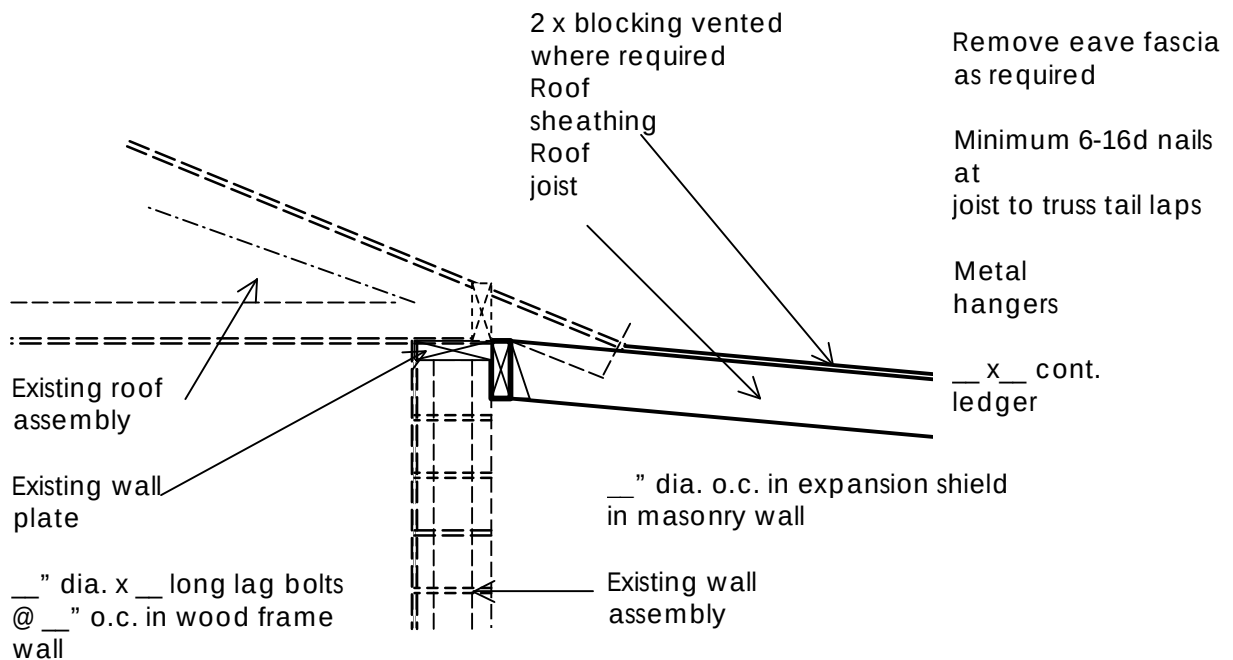
DETAIL B
